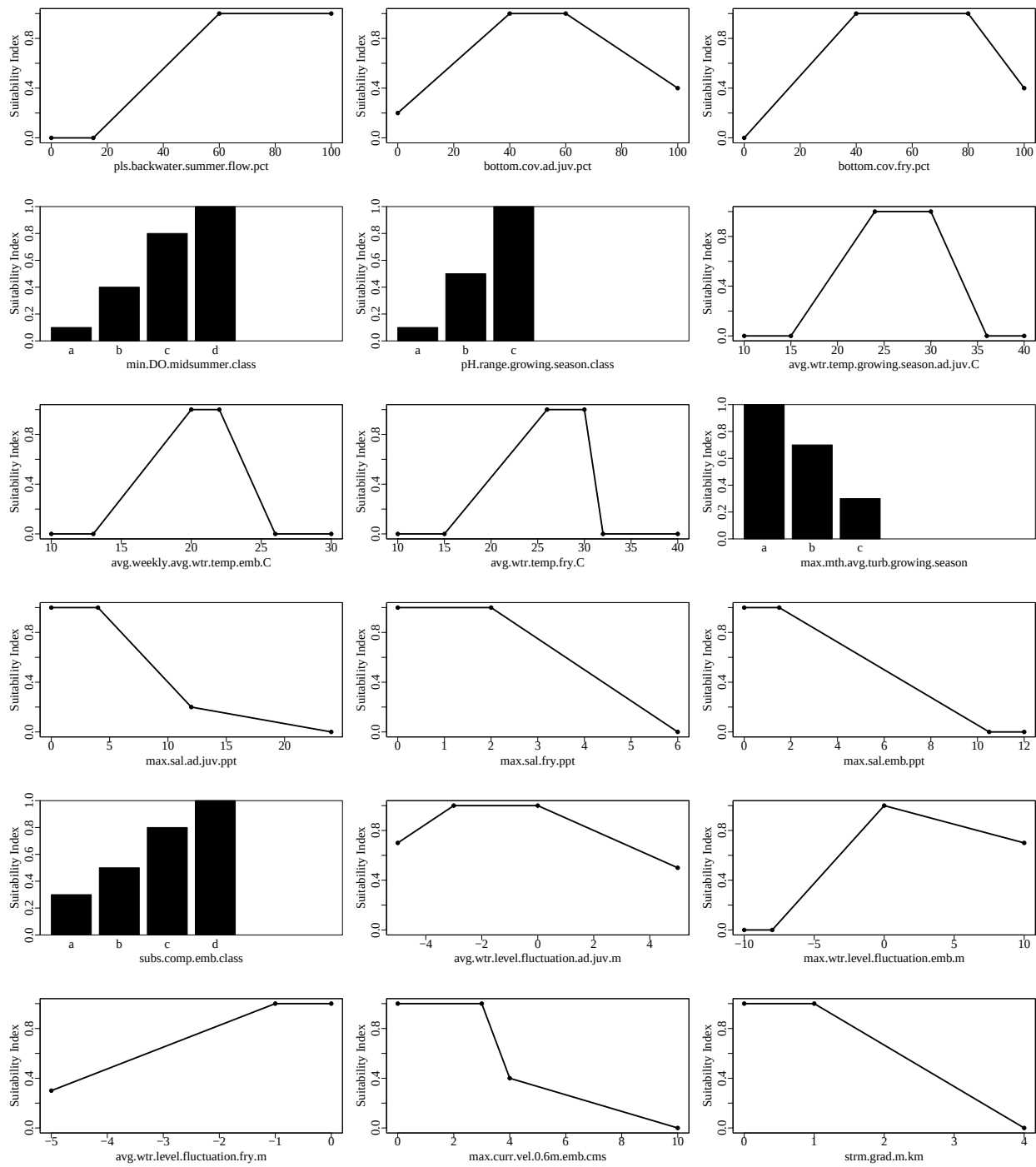
Figure 1. Suitability index graphs for variables included in the largemouthbassRivGrad model in ecorest.
